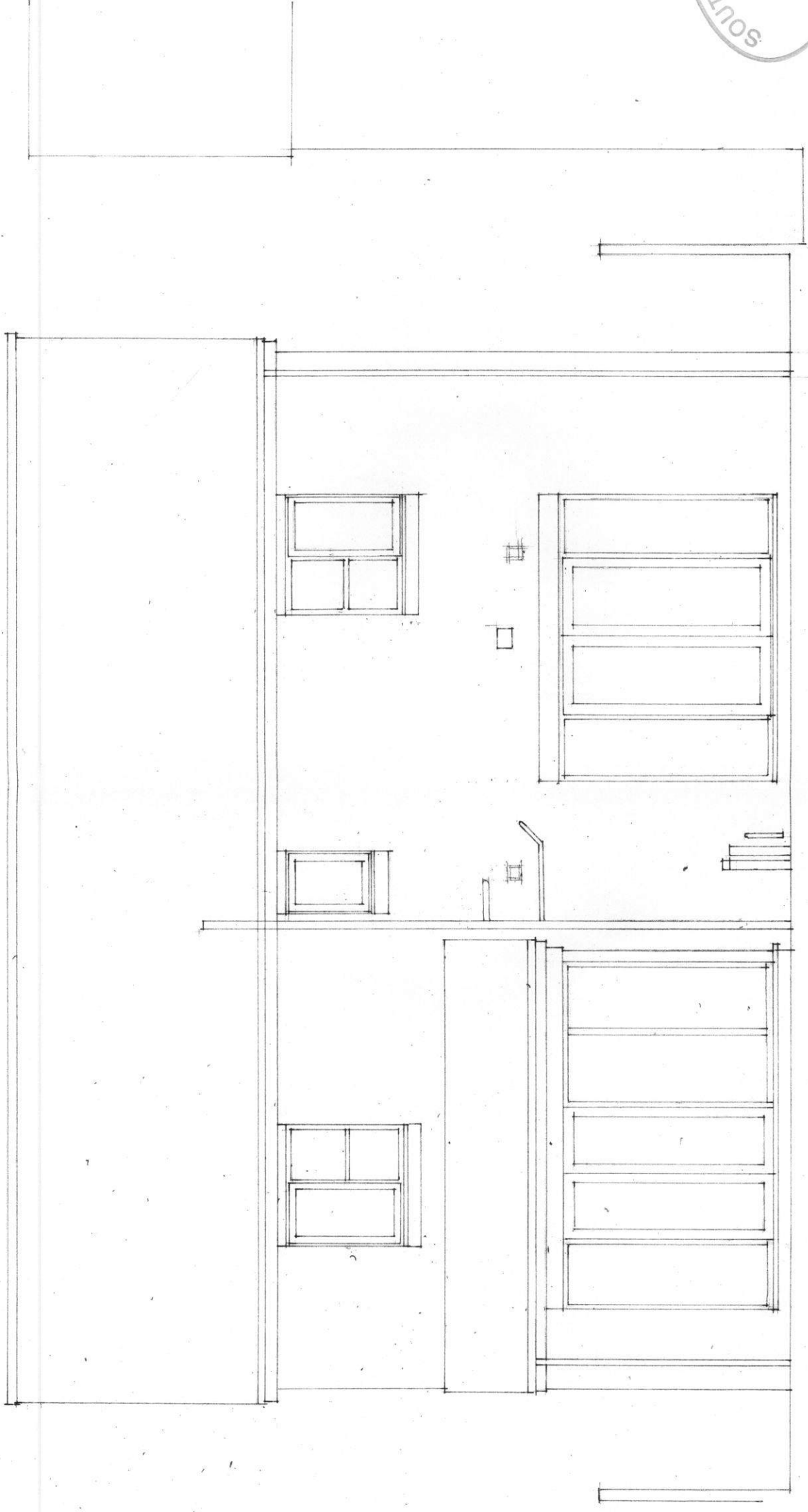
EAST ELEVATION
